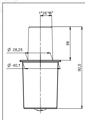
Swivel adaptor Part No 20W173
